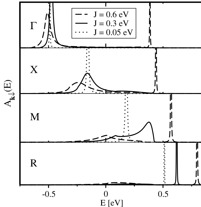
Figure 1. \downarrow -spectral density as function of energy for several symmetry points in the first Brillouin zone and for different exchange couplings J . Parameters: S = \frac{1}{2} , W = 1\text{eV} , sc lattice.
