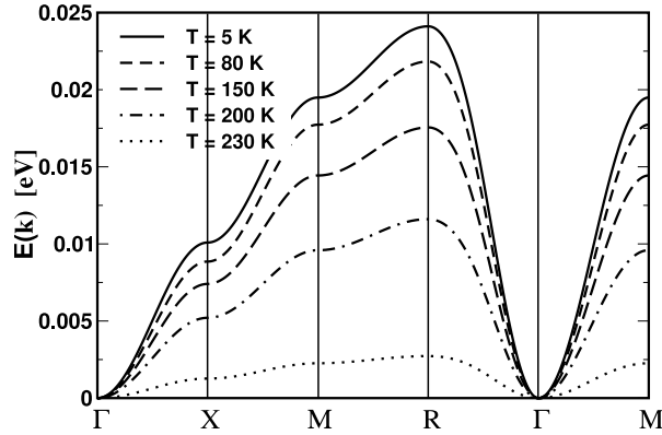
Figure 5. Spin-wave dispersion of the ferromagnetic Kondo-lattice model as a function of the wave-vector for different temperatures T . Parameters: J = 0.2 eV, n = 0.2 , S = 7/2 , sc lattice, and W = 1 eV. The self-consistently calculated Curie temperature is T_C = 232 K.
