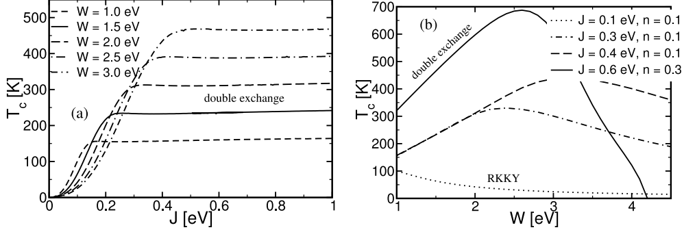
Figure 4. Curie temperature as a function of (a) the interband exchange J for various W and n = 0.1 , (b) the Bloch bandwidth W for various J and n , calculated by use of the modified RKKY.
