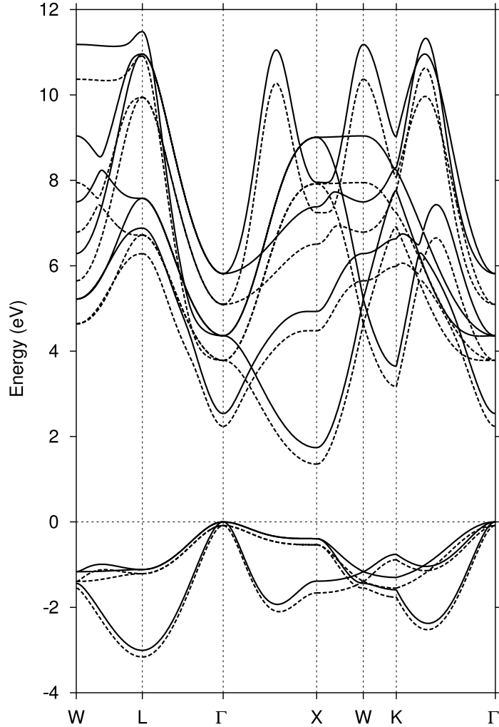
Figure 6. Spin-dependent (solid lines down-spin, broken lines up-spin) band structure of bulk EuS calculated within a TB-LMTO scheme with the 4f levels treated as core states. The energy zero coincides with the Fermi energy.
