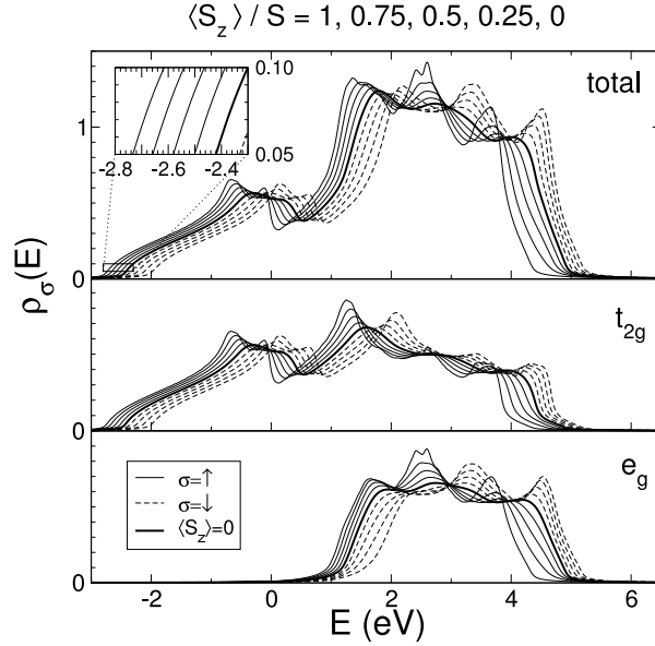
Figure 8. The same as in Fig. 7 but for bulk EuS ( J = 0.23 eV).
