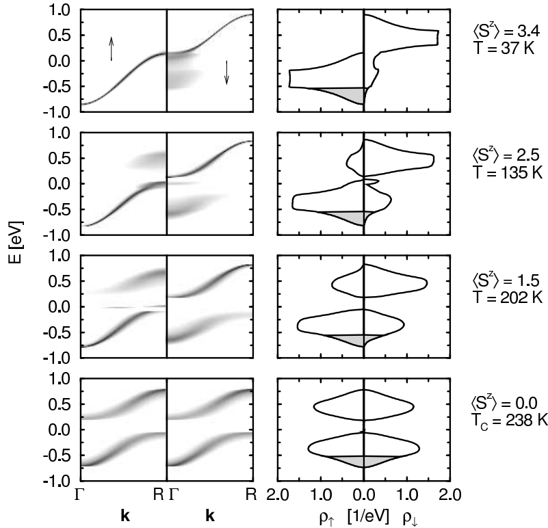
Figure 2. Quasiparticle bandstructure as a function of wave-vector (left column) and quasiparticle density of states as a function of energy (right column) for four different temperatures calculated within the MCDA[11]. Parameters: J = 0.2 eV, W = 1 eV, n = 0.2 , S = \frac{7}{2} , sc lattice.
