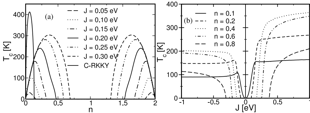
Figure 3. Curie temperature as a function of (a) the band occupation n for various J , (b) the interband exchange coupling J for various n , calculated by use of the modified RKKY.
