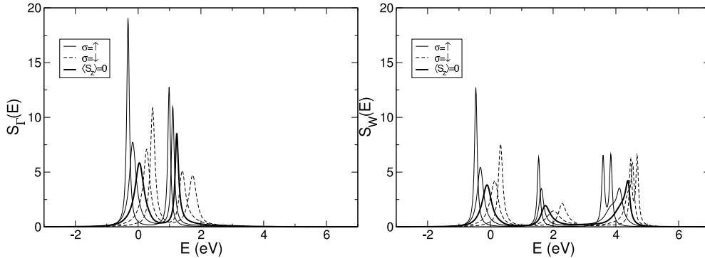
Figure 10. (a) Spin-dependent spectral density S_{\mathbf{k}\sigma} for \mathbf{k} from the \Gamma -point (5d states) of bulk EuS ( J = 0.23 eV) as a function of the energy for three different 4f magnetizations: \langle S_z \rangle / S = 1.0, 0.5, 0 . Thick line for T = T_C . Solid lines: up-spin; broken lines: down-spin. Curves with maximum spin splitting of the peaks belong to T = 0 . (b) The same as in (a) but for the W-point.
